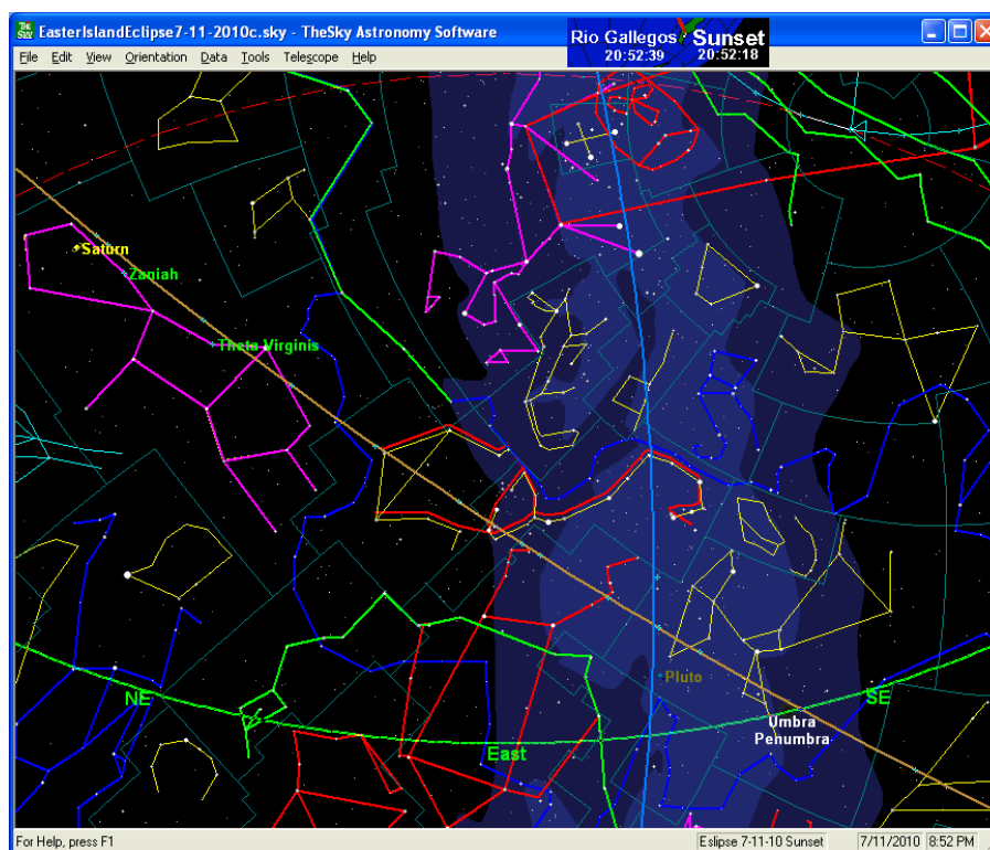
Figure 79: Sunset East03
