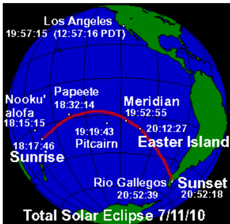
Figure 33: Solar Eclipse 7-11-10
