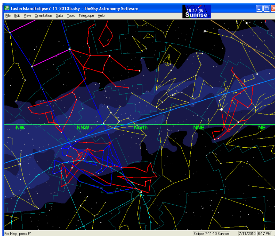
Figure 52: Sunrise North2
