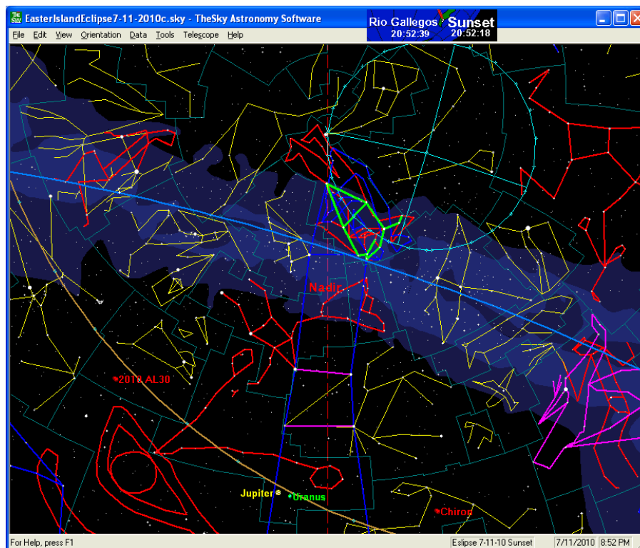
Figure 72: Sunset Nadir4
