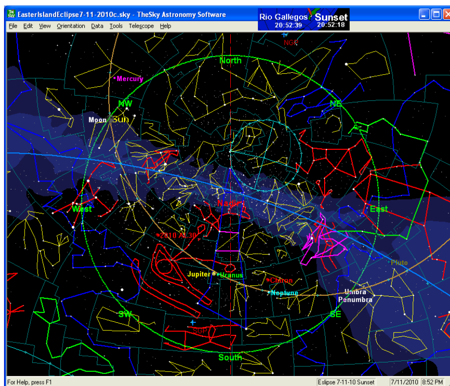
Figure 69: Sunset Nadir1
