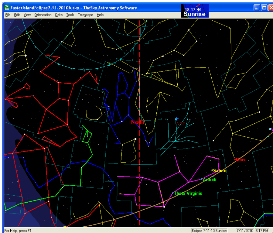
Figure 48: Sunrise Nadir2
