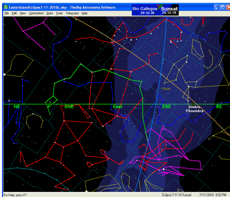
Figure 77: Sunset East01
