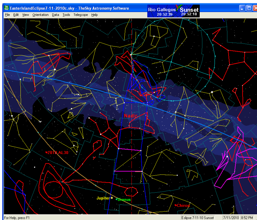
Figure 73: Sunset Nadir5
