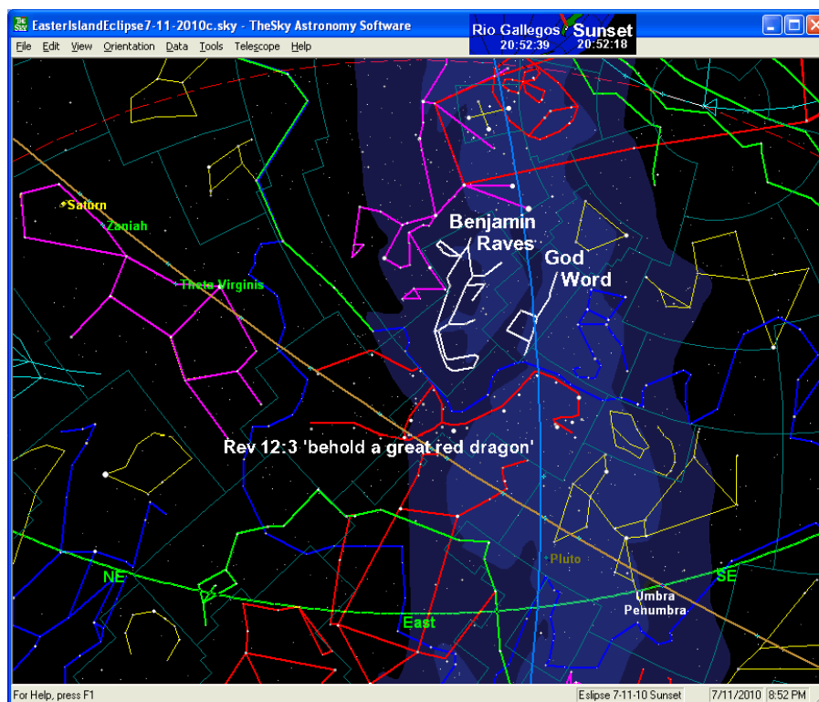
Figure 80: Sunset East04
