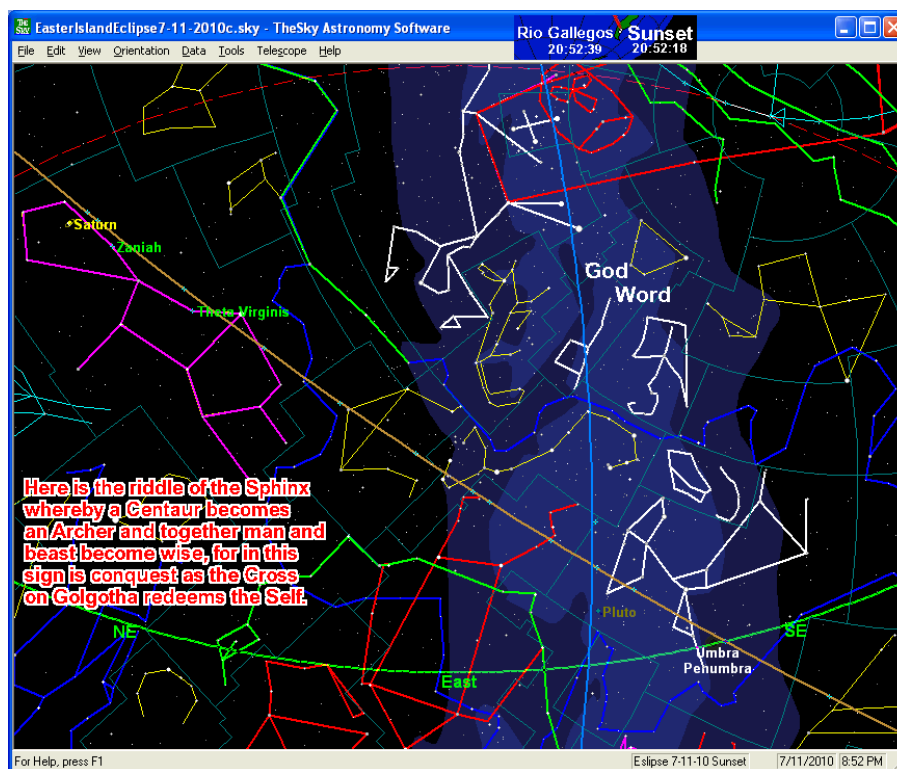
Figure 86: Sunset East10
