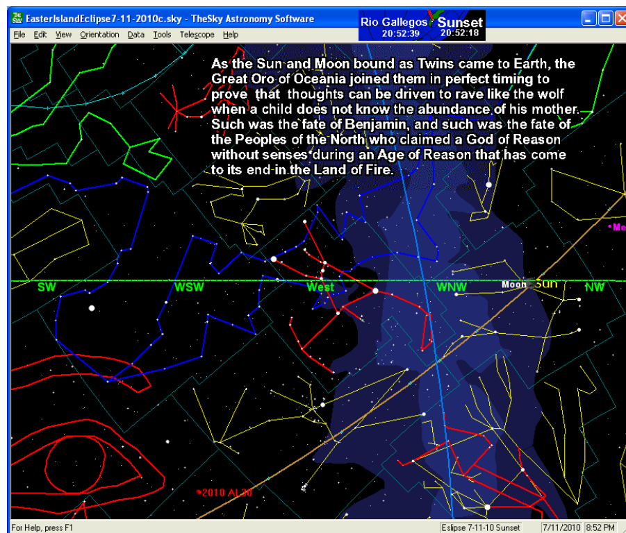
Figure 75: Sunset West1
