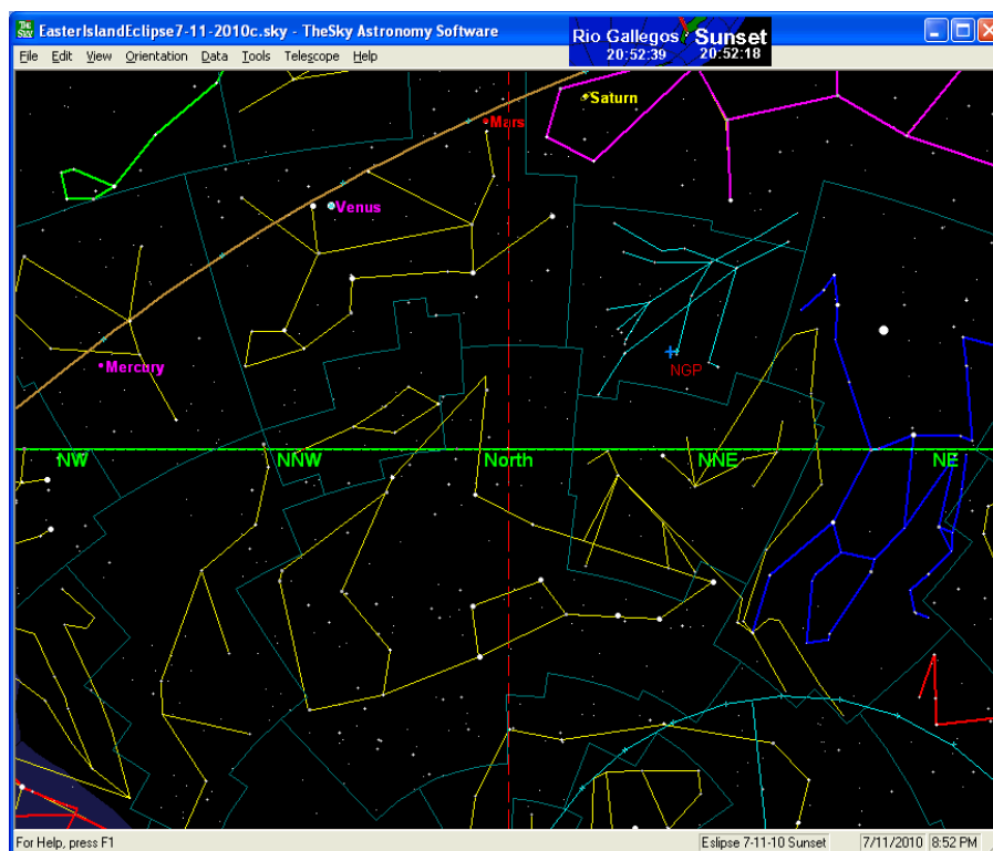
Figure 76: Sunset North1
