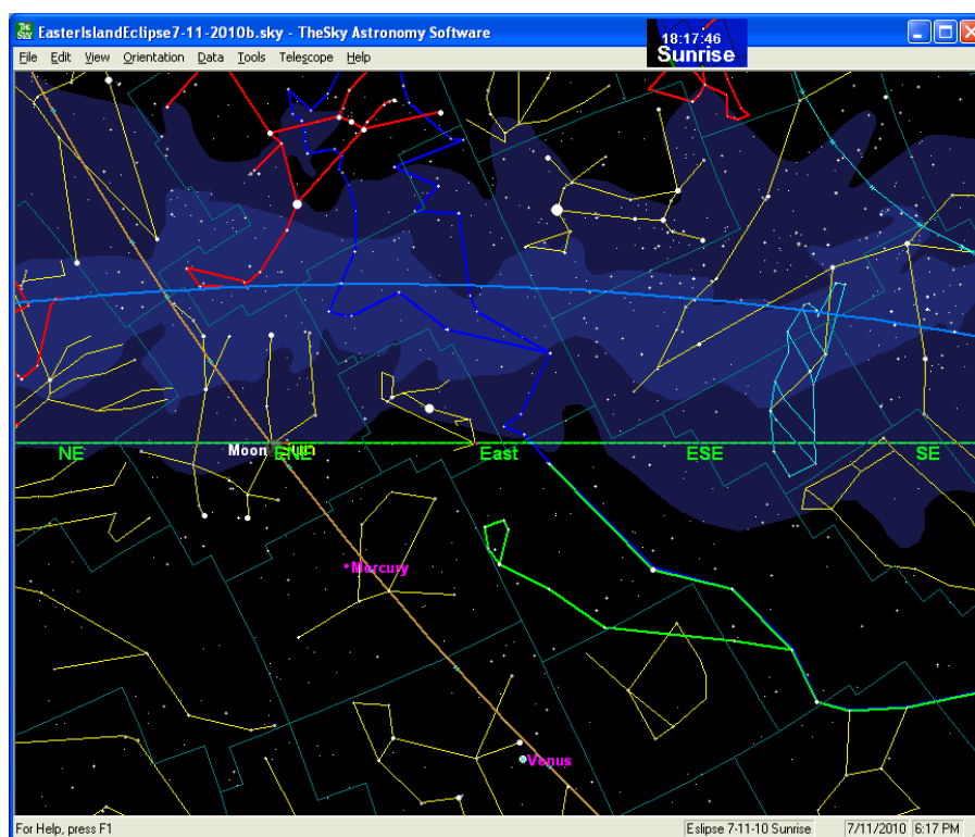
Figure 53: Sunrise East1
