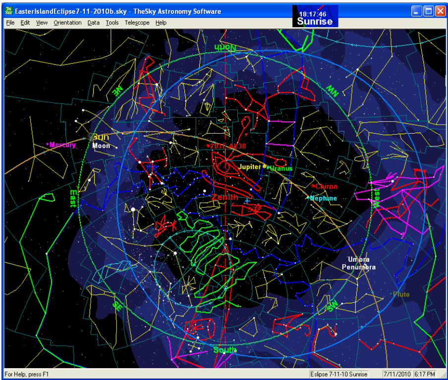
Figure 45: Sunrise Zenith1
