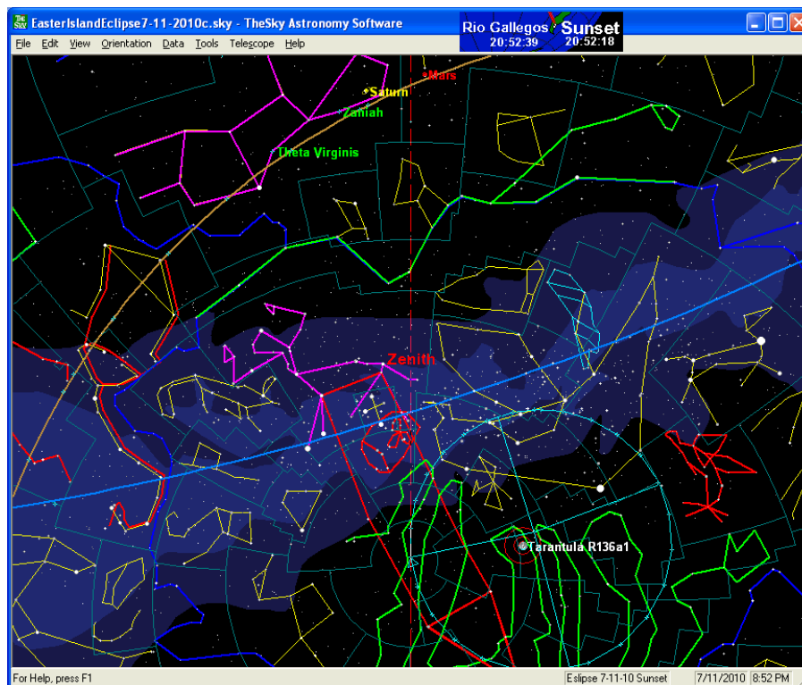
Figure 66: Sunset Zenith2
