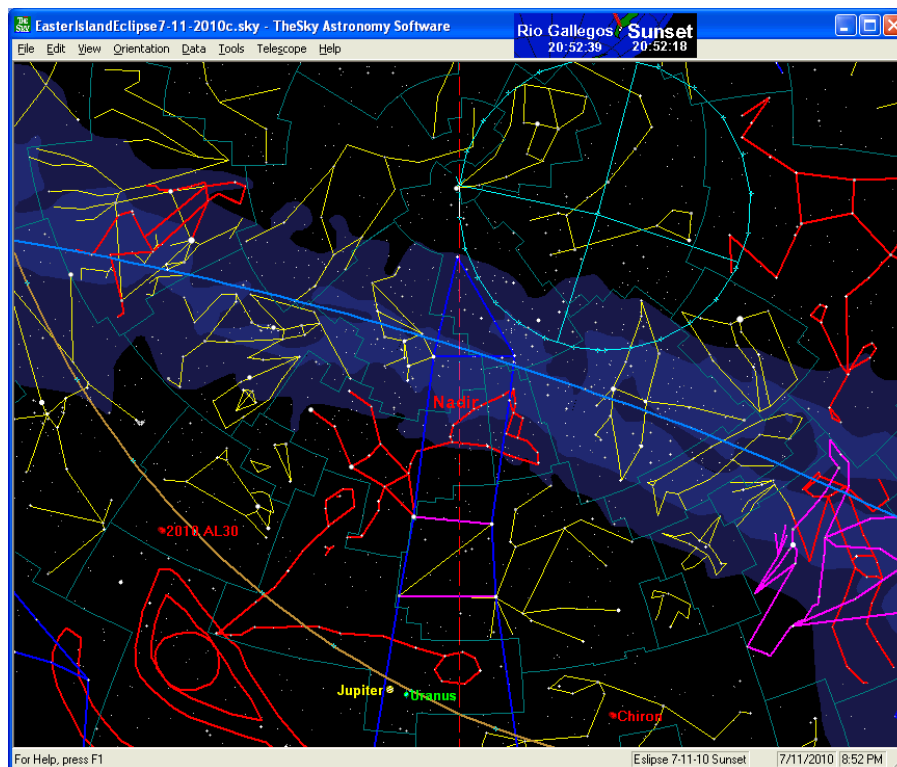
Figure 70: Sunset Nadir2
