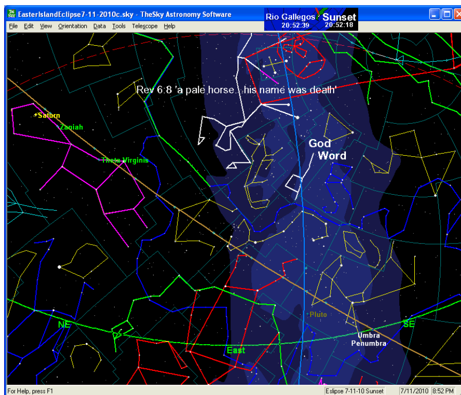
Figure 84: Sunset East08
