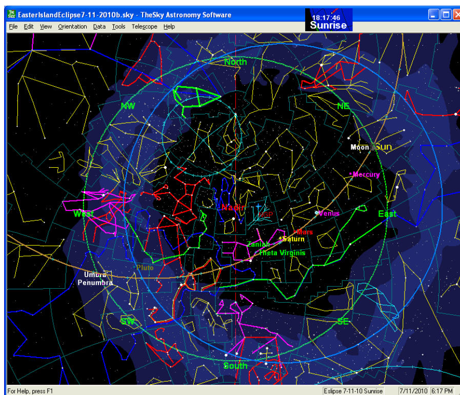
Figure 47: Sunrise Nadir1
