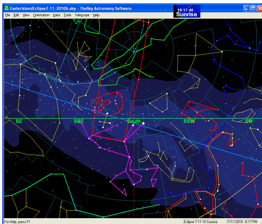
Figure 49: Sunrise South1
